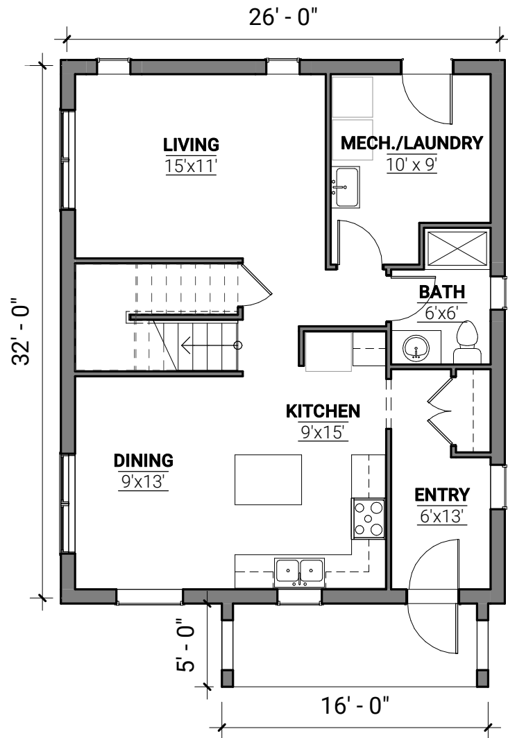
Schematic First Floor Plan 870 square feet
