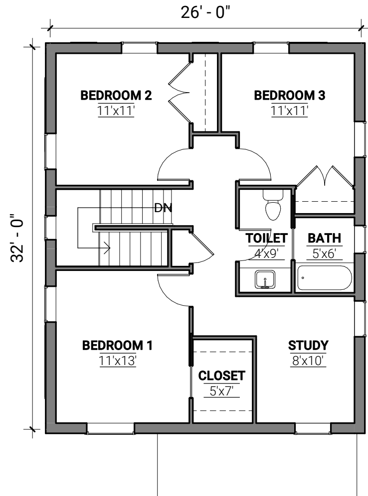
Schematic Second Floor Plan 870 square feet
